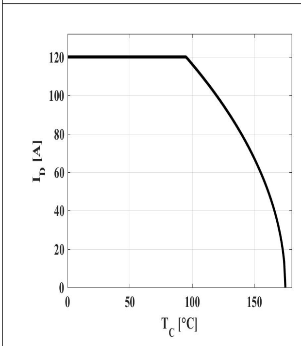
Figure 5: Drain Current
