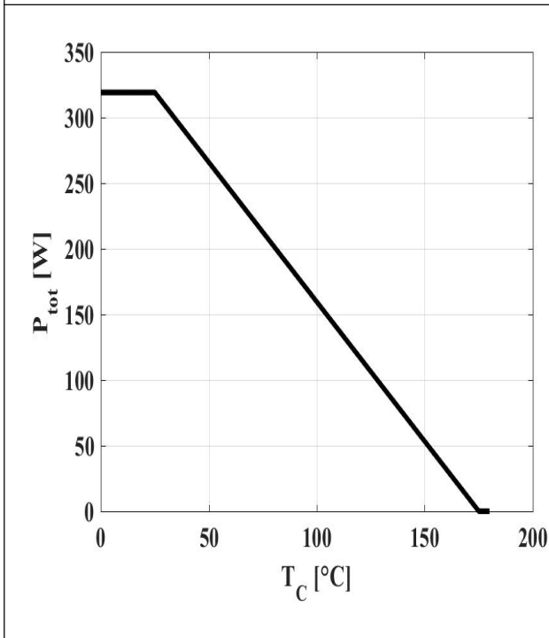
Figure 3: Power Dissipation
