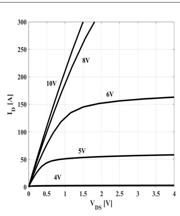
Figure 6: Typ. Output Characteristics
