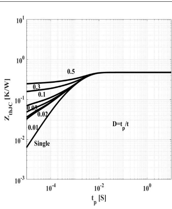
Figure 4: Max. Transient Thermal Impedance
